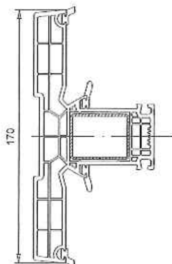
Handrahmen 101.303 Stahl 113.023
